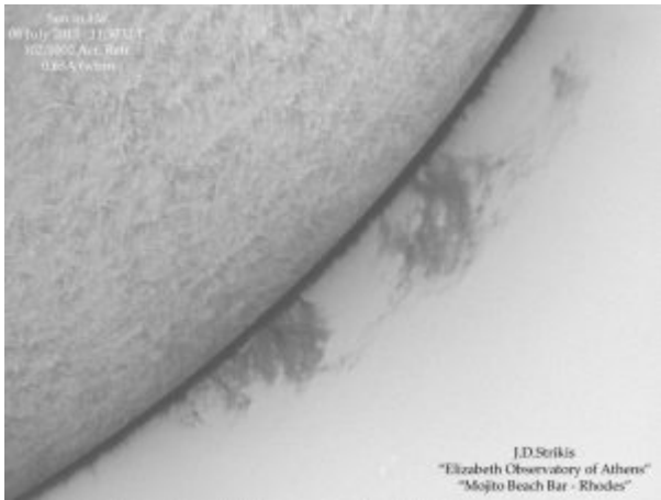
Solar Prominences in Ha' line by Iakovos Strikis
